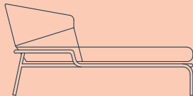
ROCK SUN LOUNGER ERP Code L02091201 cm w105 x d164 x h80/sh40 inch w41.3 x d64.6 x h31.5/sh15.7
